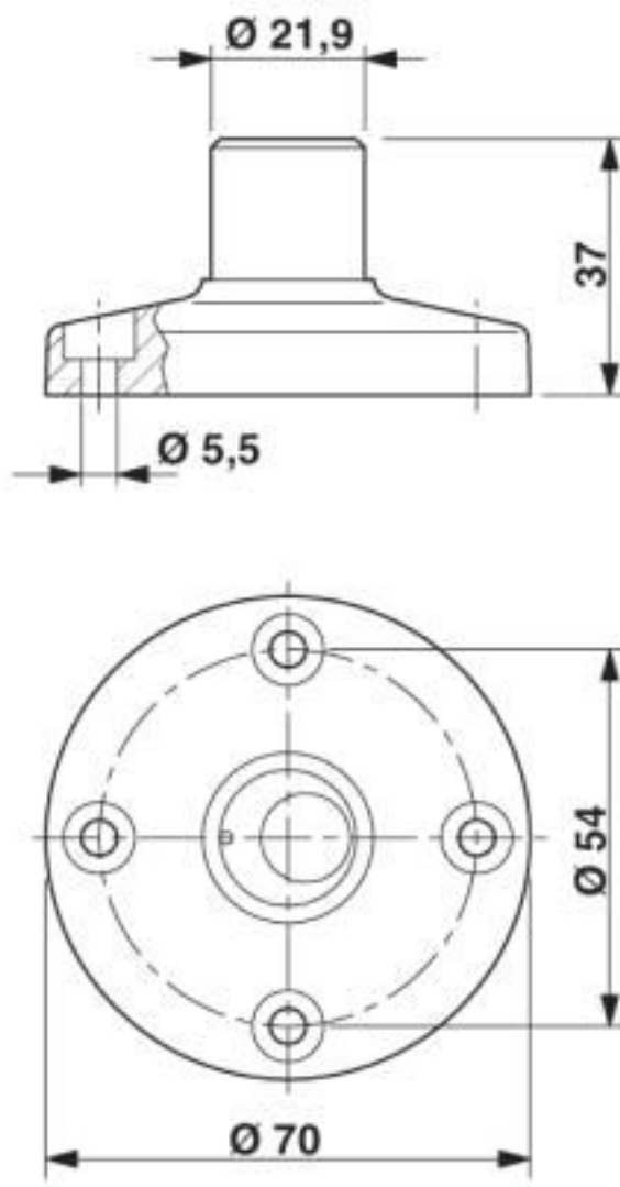
Dimensional drawing
