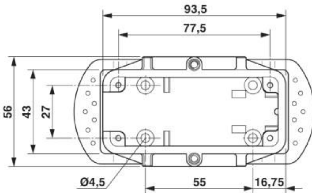
Dimensional drawing top view
