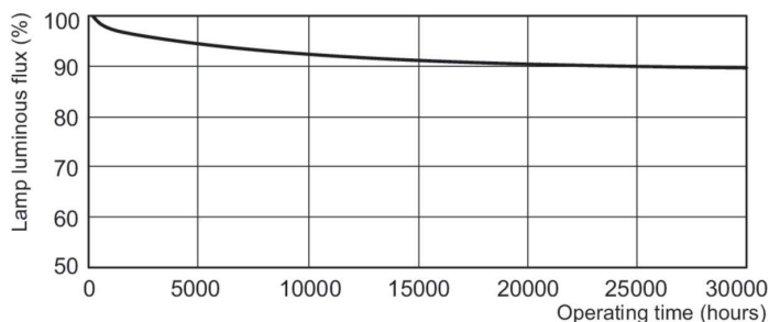
Lumen Maintenance Diagram - MASTER TL5 HO 90 De Luxe 49W/952
