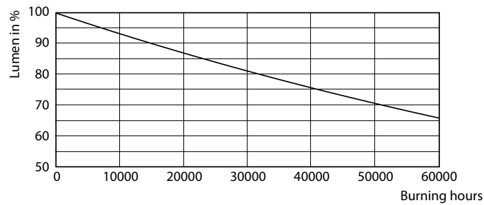
Lumen Maintenance Diagram - TForce LED Road 84-55W E40 730
