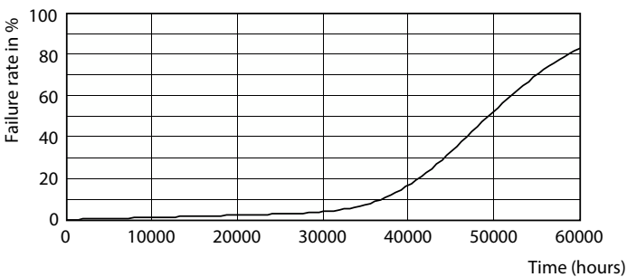
Life Expectancy Diagram - TForce LED Road 84-55W E40 730
