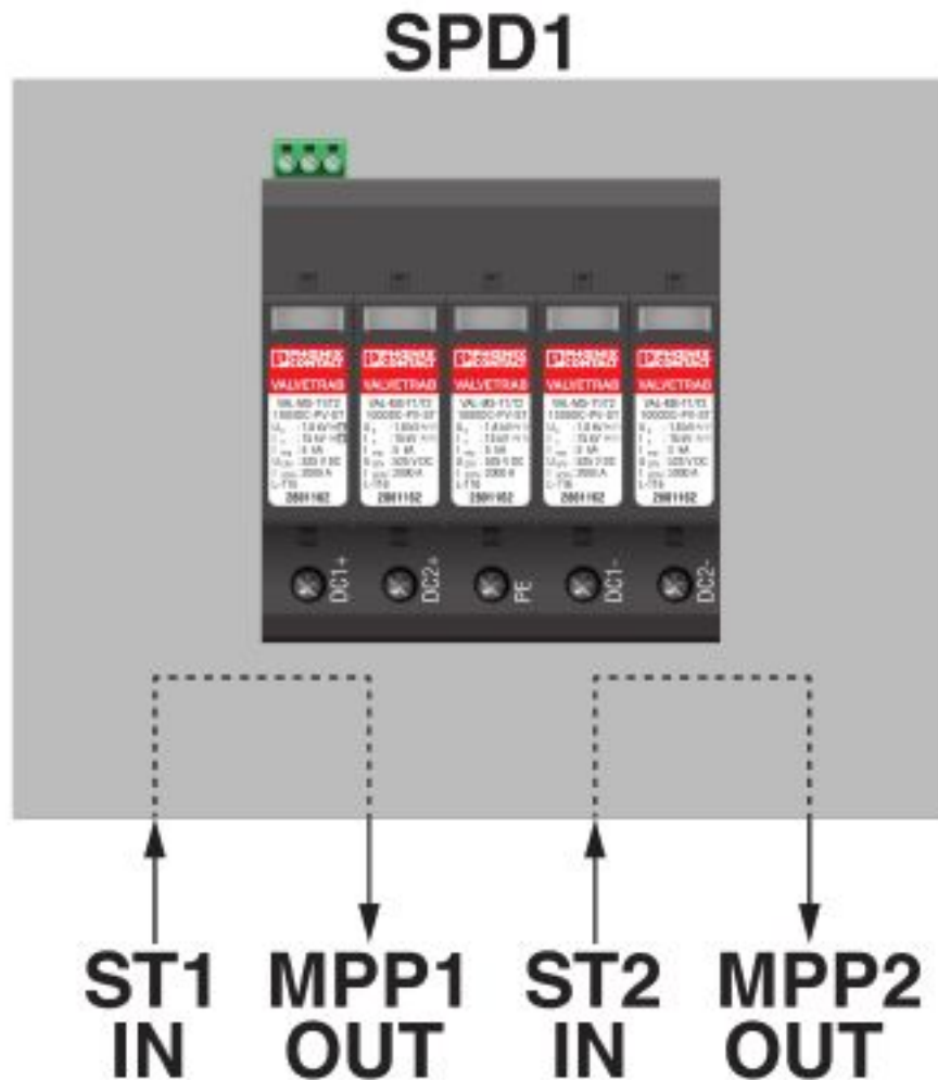
Connection diagram
