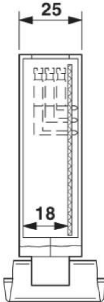
Dimensional drawing
