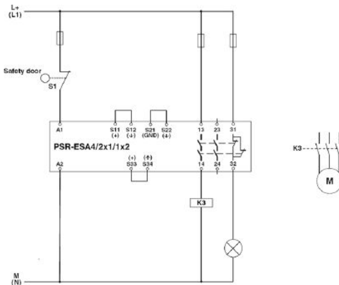
Circuit diagram
