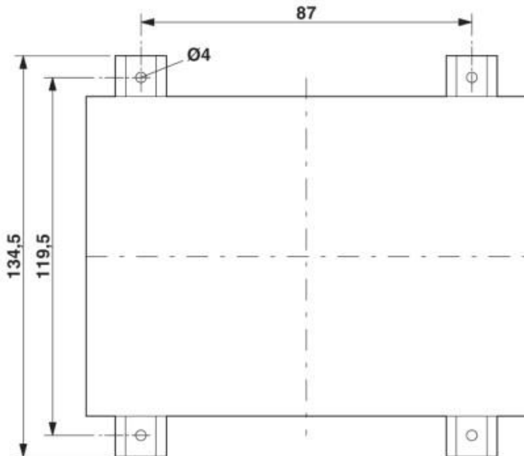
Dimensional drawing
