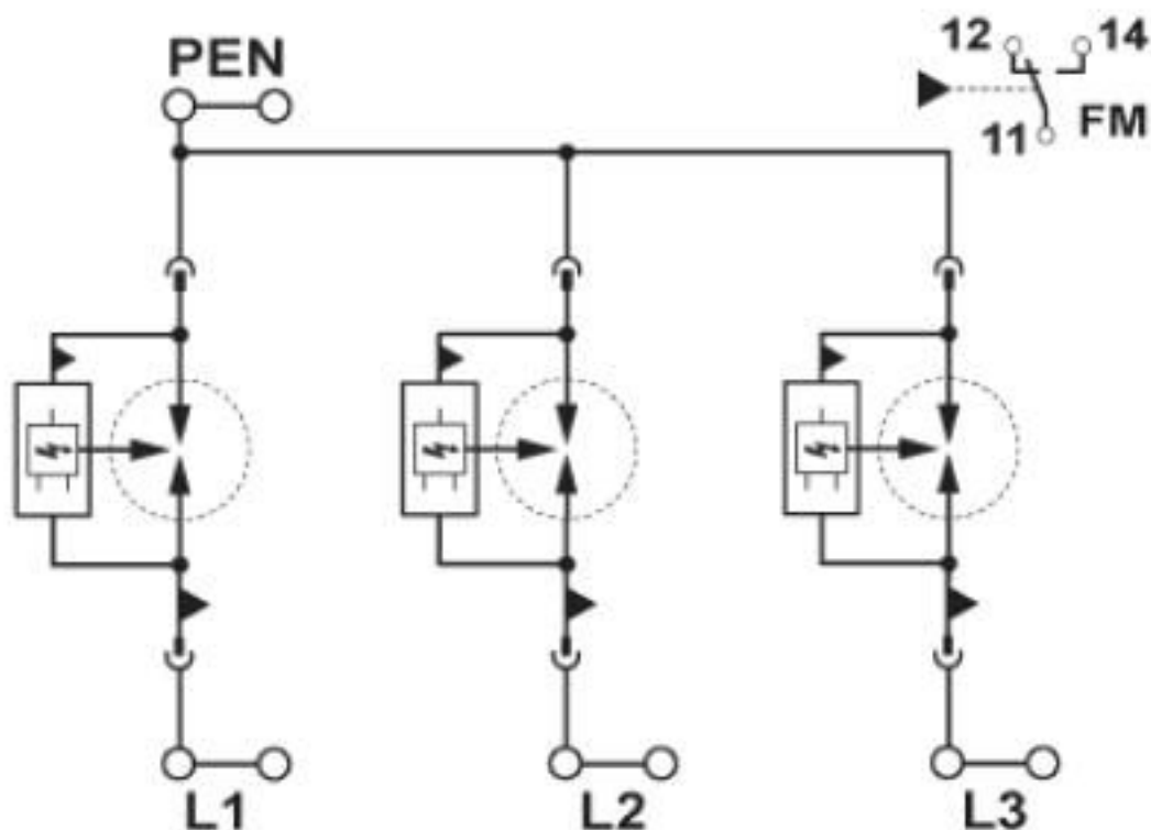
Circuit diagram
