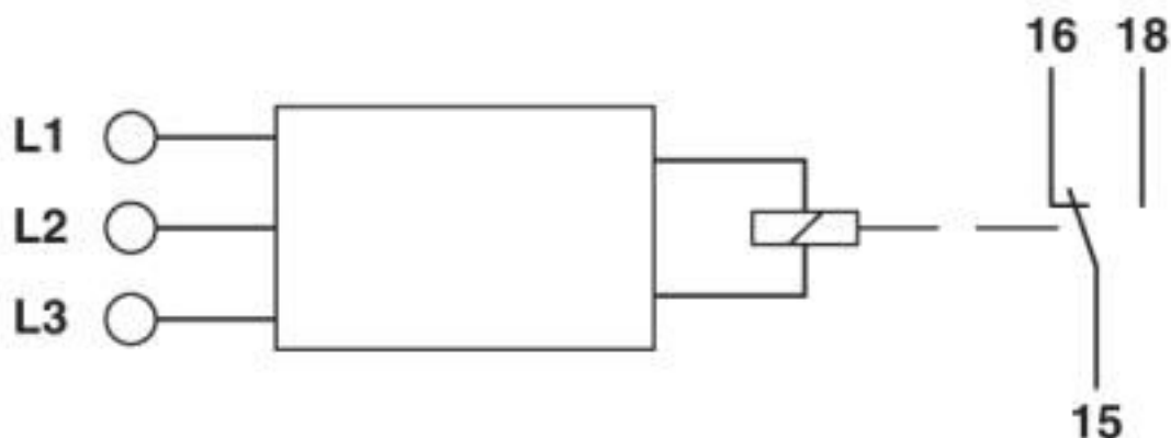
Block diagram
