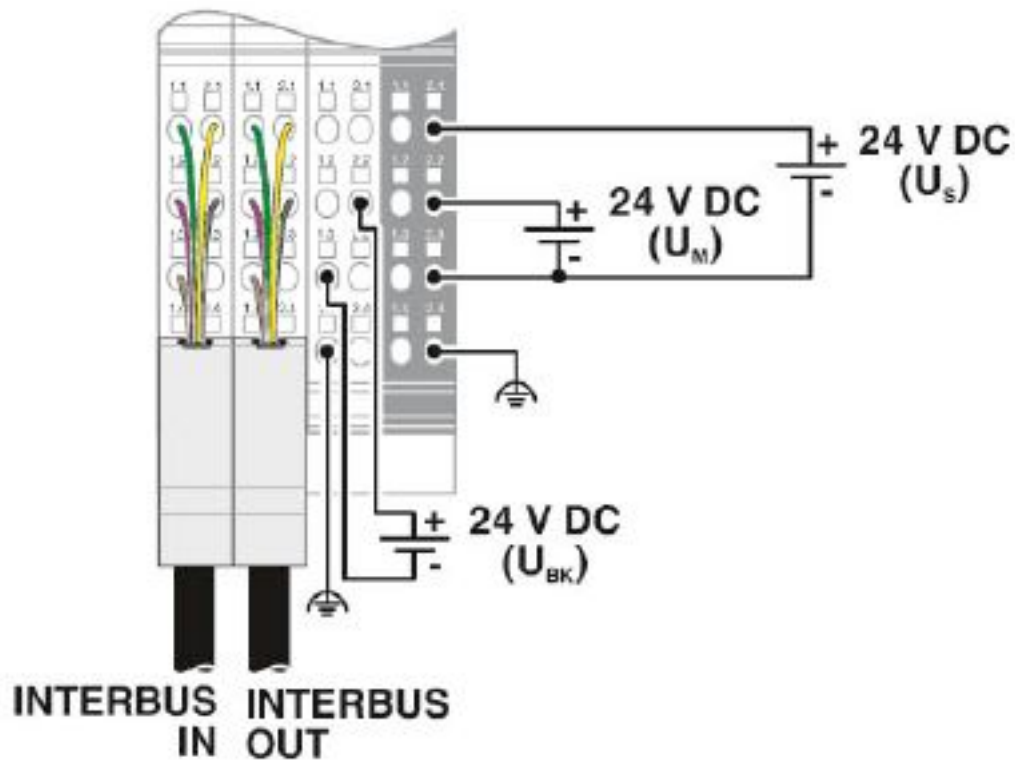
Block diagram
