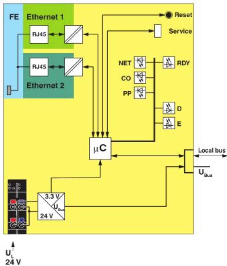
Block diagram
