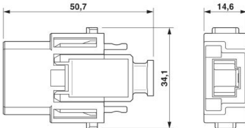
Dimensional drawing
