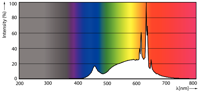
Spectral Power Distribution Colour - MAS LED spot VLE D 650lm GU10 930 120D
