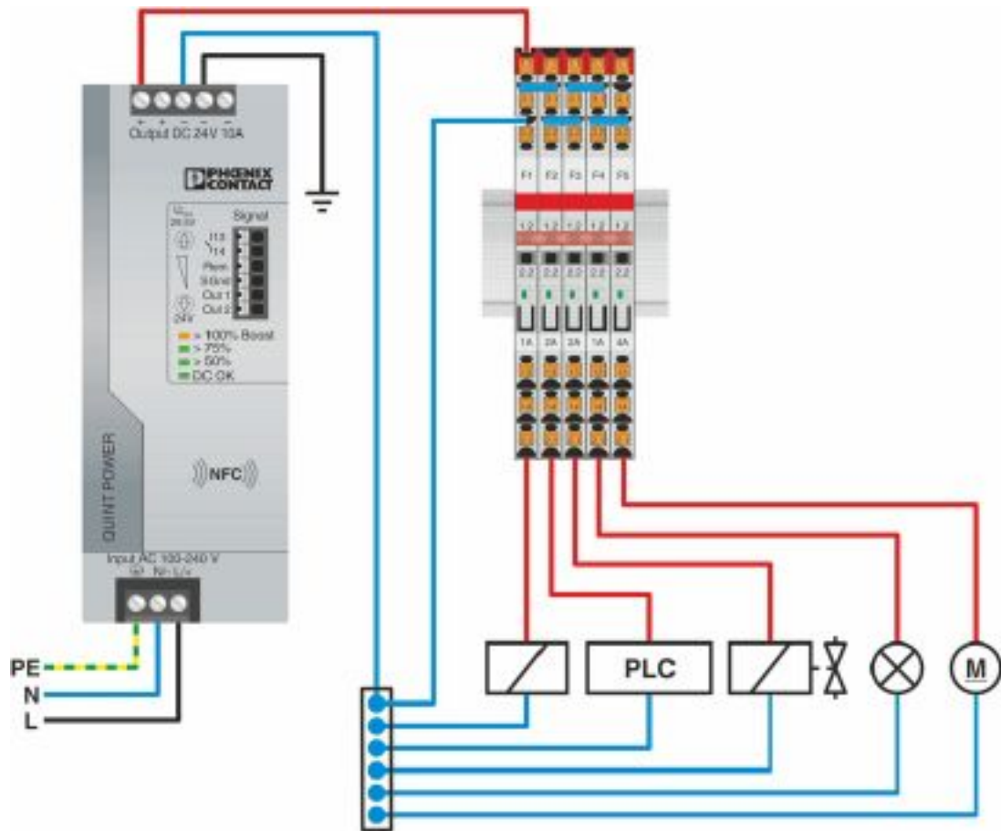
Application drawing
