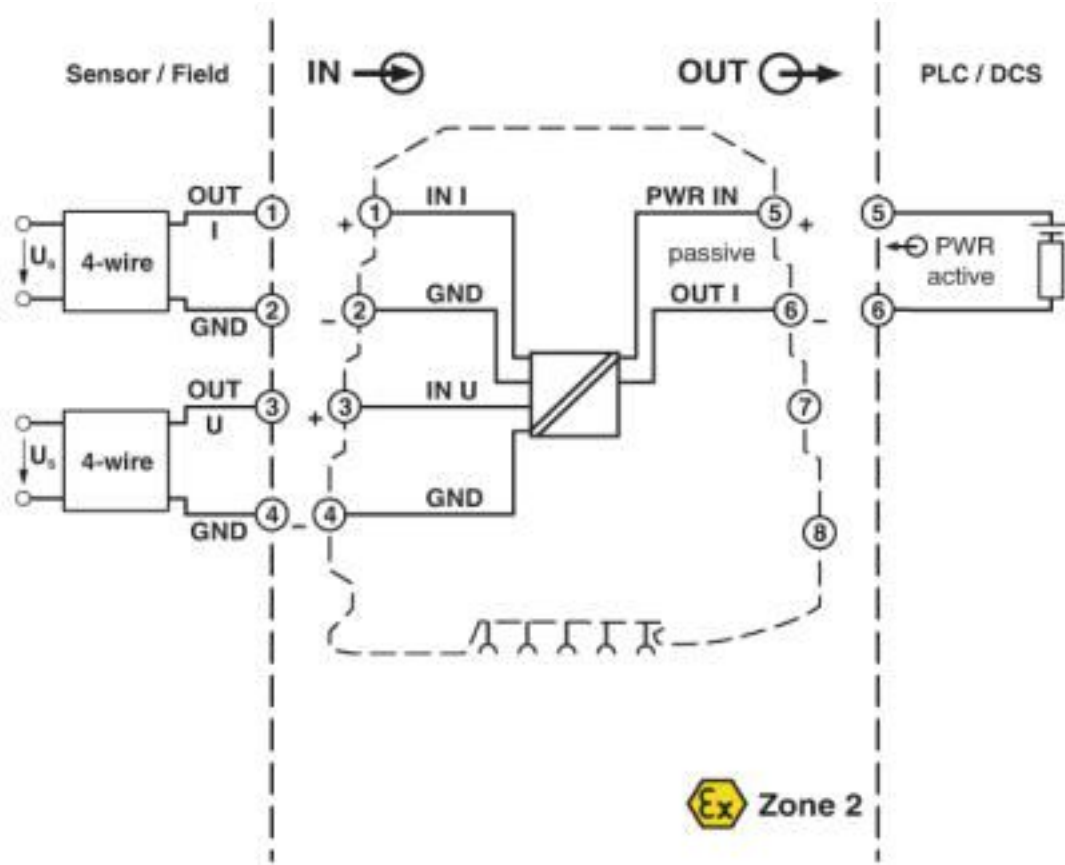
Block diagram
