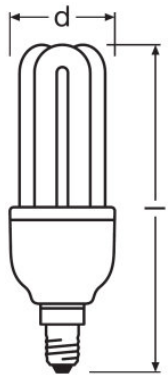
D STICK 11 W/2700K 220...240 V E14, D STICK 11 W/4000K 220...240 V E14, D STICK 11 W/6500K 220...240 V E14
